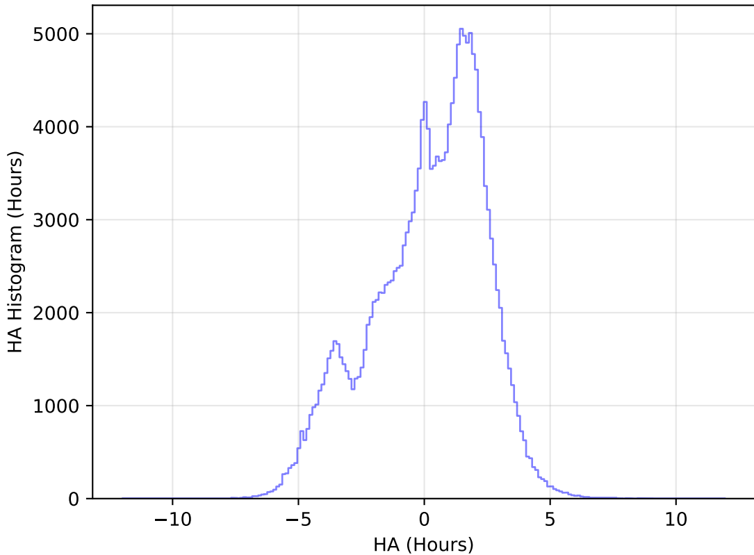
internal_u_expt38_nscale1.1v3.4_10yrs All sky g band: HA Histogram
