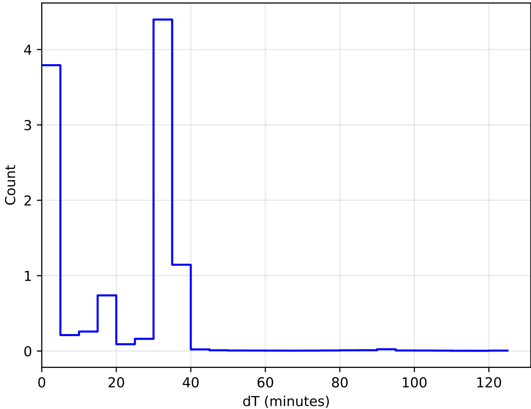
internal_u_expt38_nscale1.1v3.4_10yrs WFD: DeltaT Histogram 1e6
