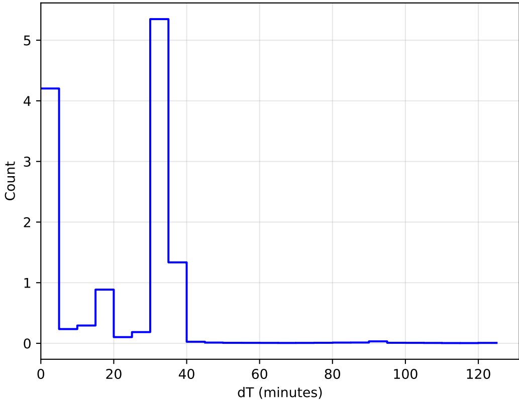
internal_u_expt38_nscale1.1v3.4_10yrs All sky: DeltaT Histogram 1e6
