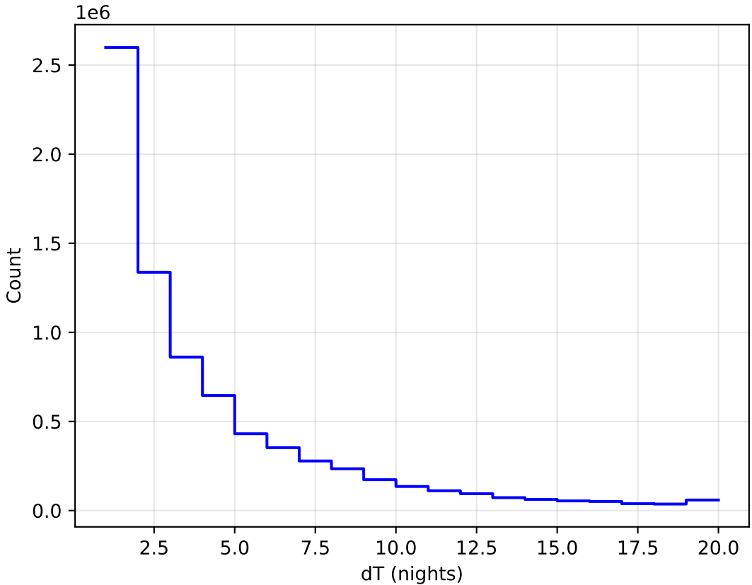
internal_u_expt38_nscale1.1v3.4_10yrs WFD all bands: DeltaNight Histogram
