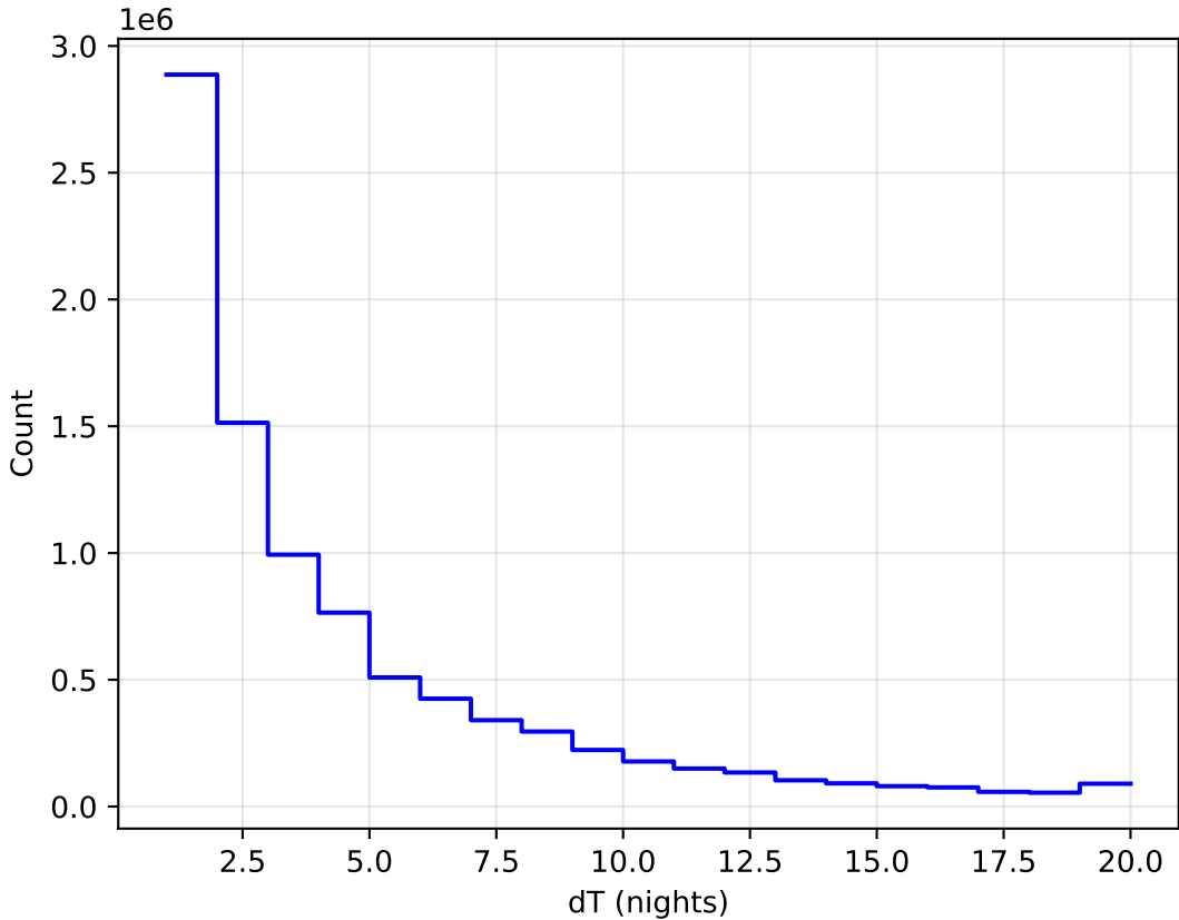
internal_u_expt38_nscale1.1v3.4_10yrs All sky all bands: DeltaNight Histogram
