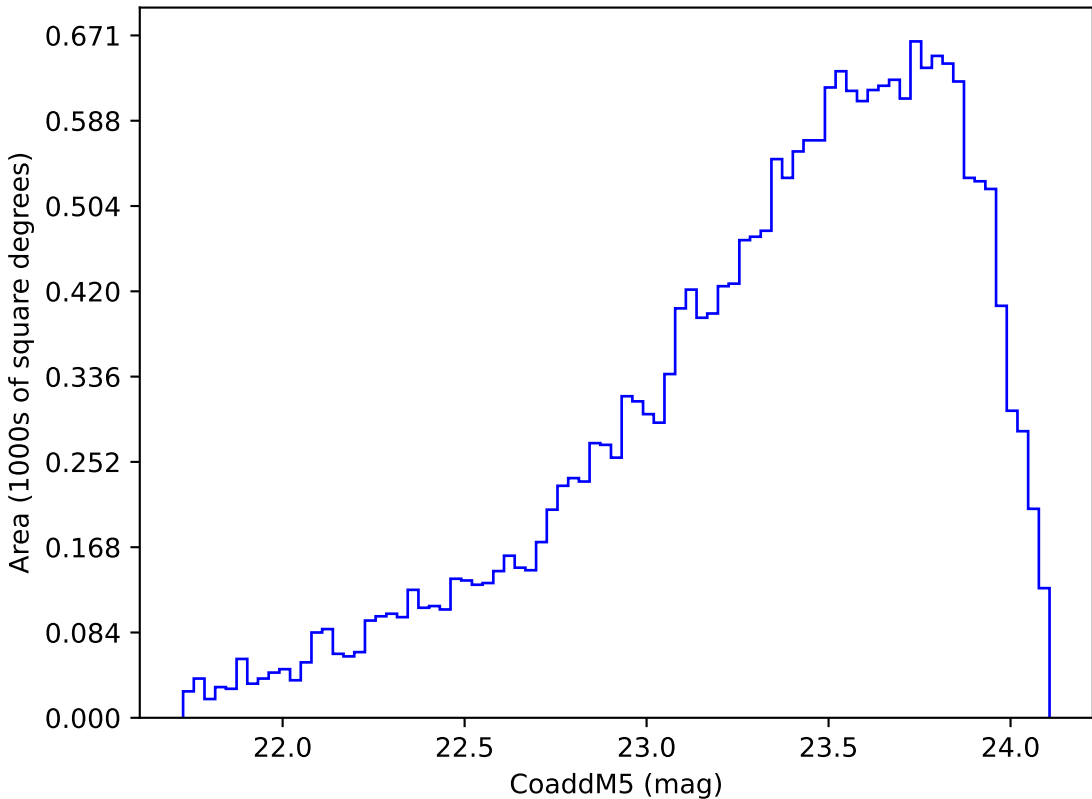
internal_u_expt38_nscale1.1v3.4_10yrs Yr 3-4 y band: CoaddM5
