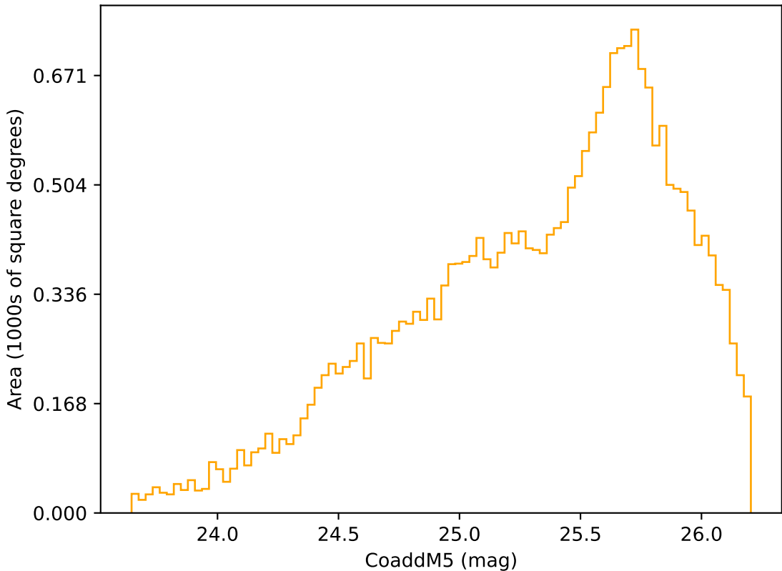
internal_u_expt38_nscale1.1v3.4_10yrs Yr 3-4 r band: CoaddM5
