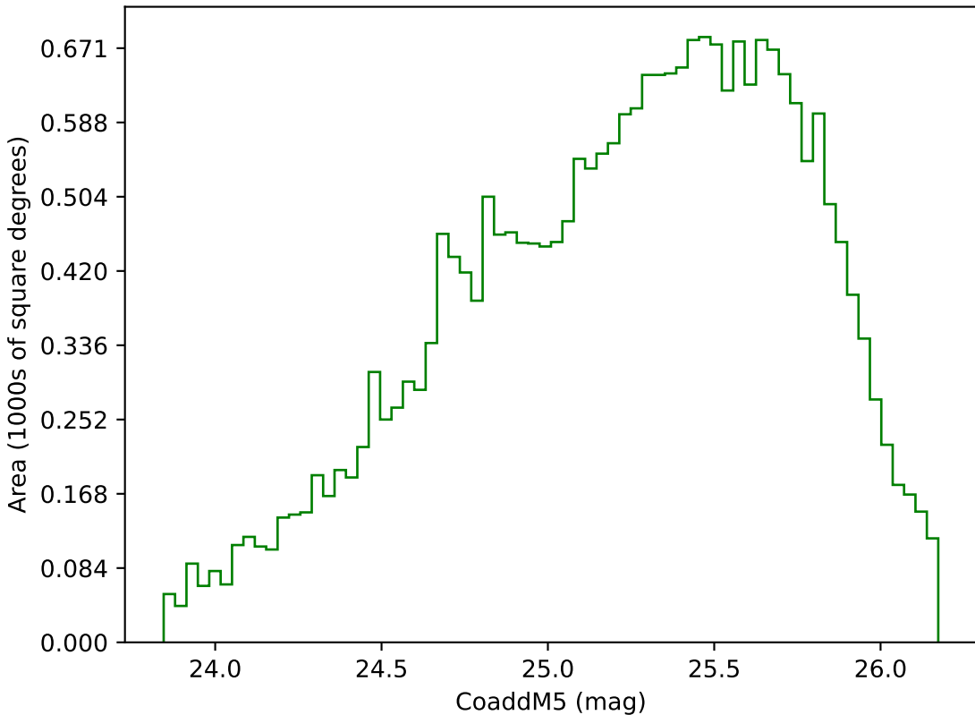
internal_u_expt38_nscale1.1v3.4_10yrs Yr 3-4 g band: CoaddM5
