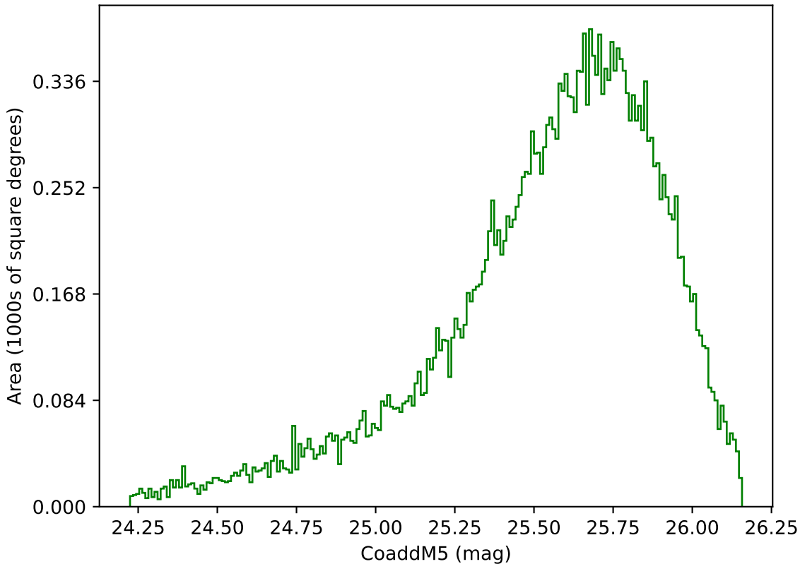
internal_u_expt38_nscale1.1v3.4_10yrs Yr 1 g band: CoaddM5
