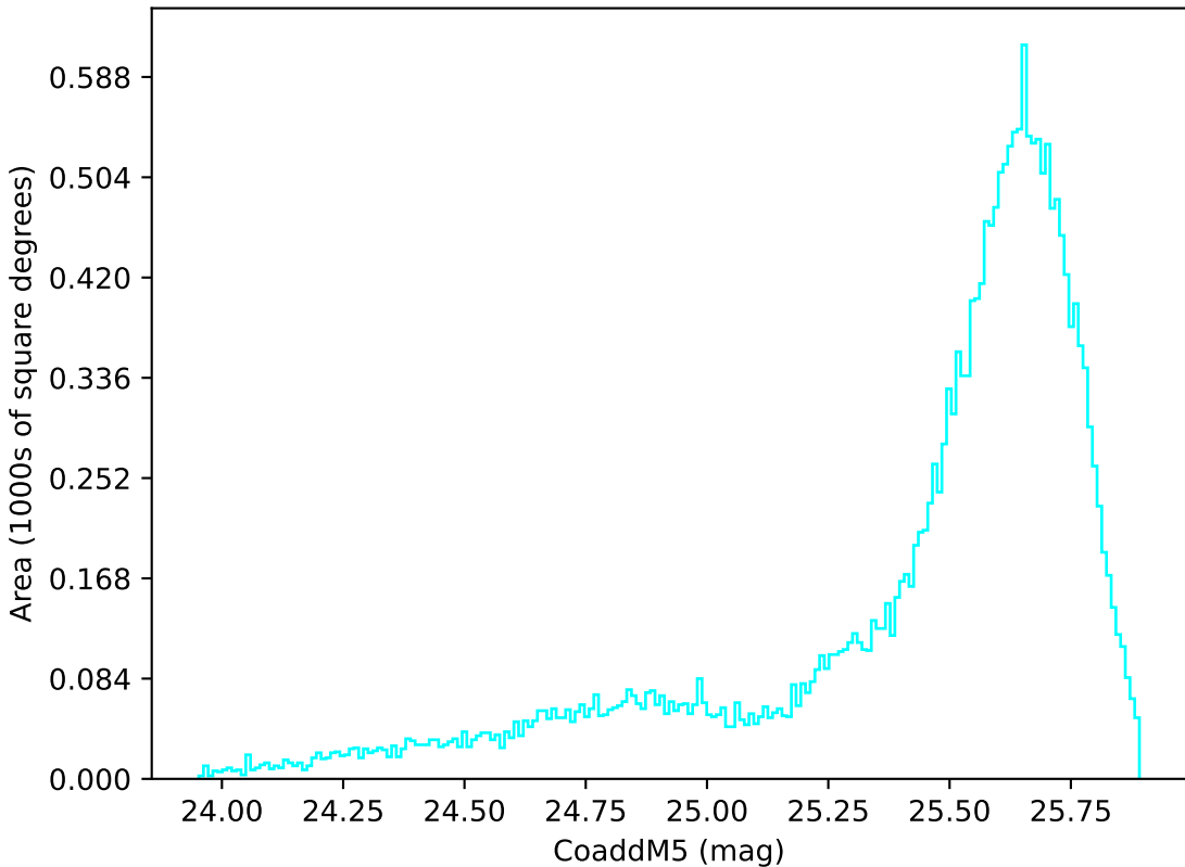
internal_u_expt38_nscale1.1v3.4_10yrs All sky u band: CoaddM5
