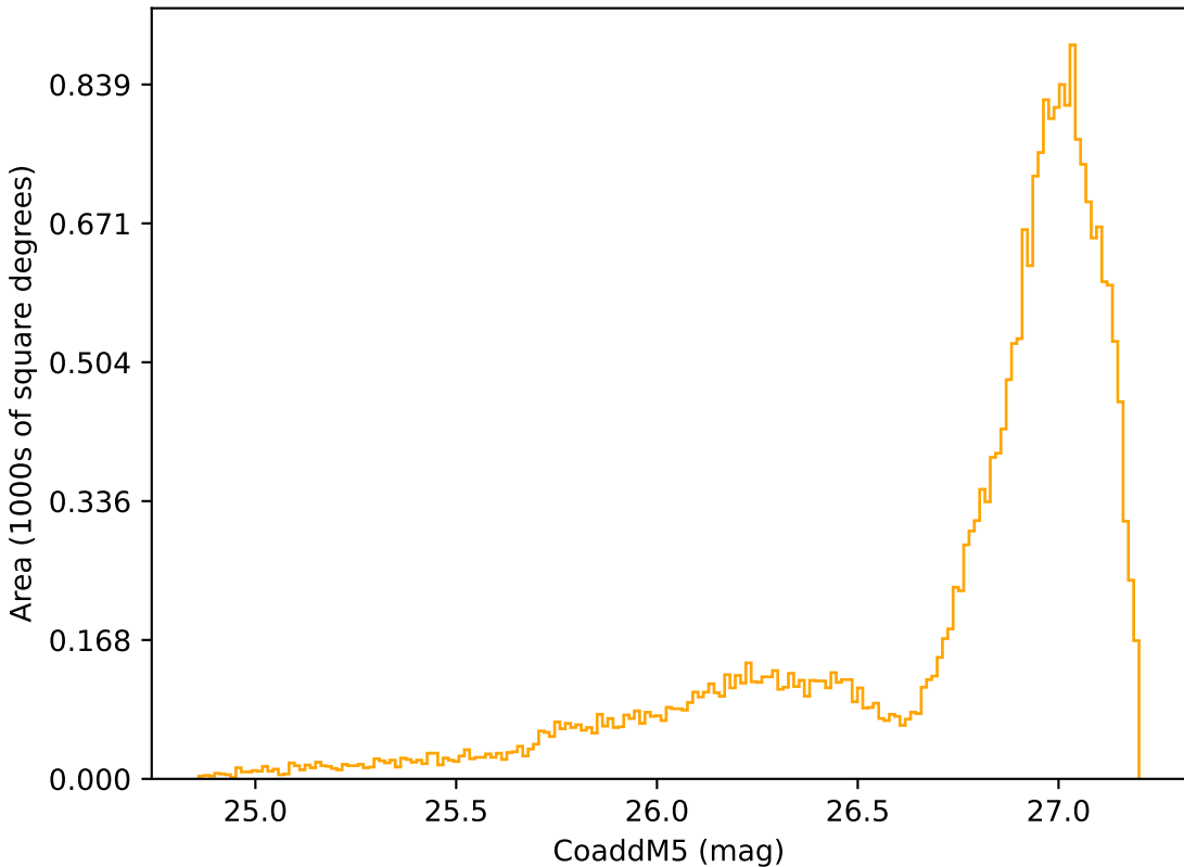
internal_u_expt38_nscale1.1v3.4_10yrs All sky r band: CoaddM5
