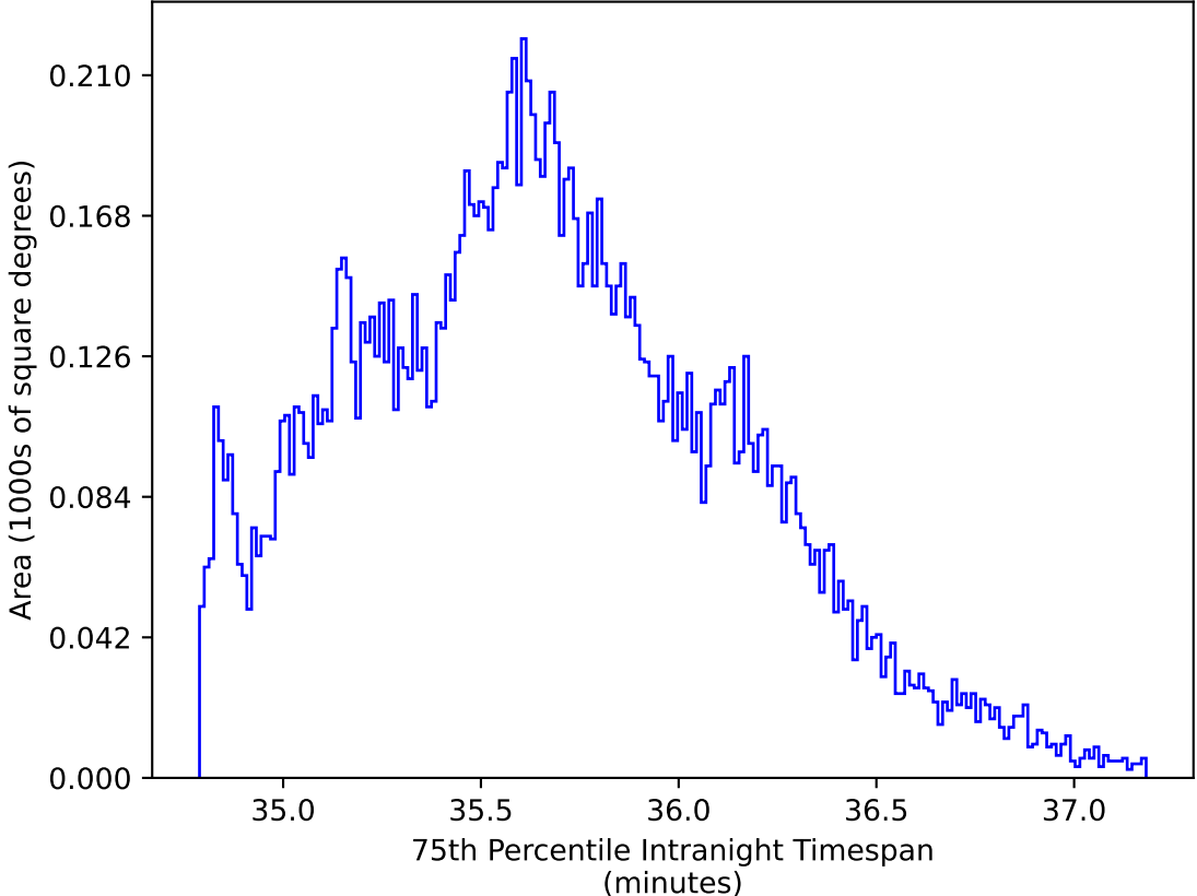
internal_u_expt38_nscale1.1v3.4_10yrs WFD: 75th Percentile Intranight Timespan
