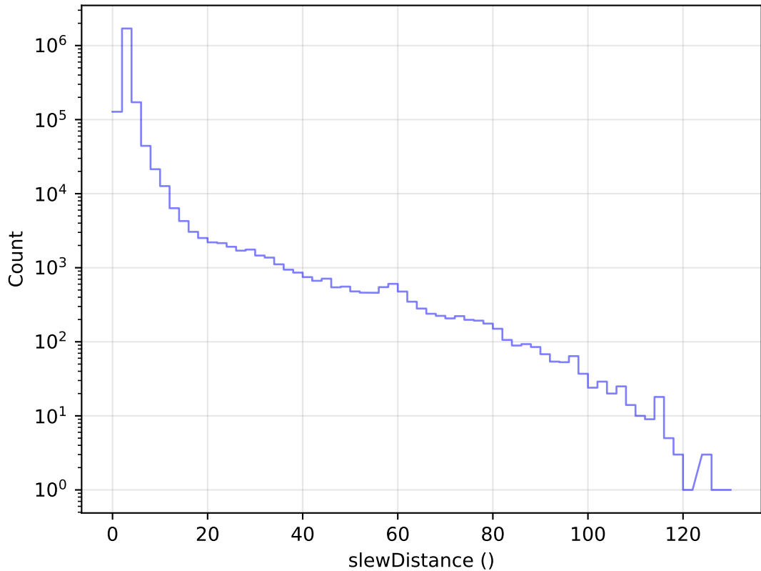
internal_u_expt38_nscale1.1v3.4_10yrs All visits: Slew Distance Histogram
