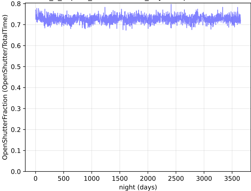
internal_u_expt38_nscale1.1v3.4_10yrs : OpenShutterFraction
