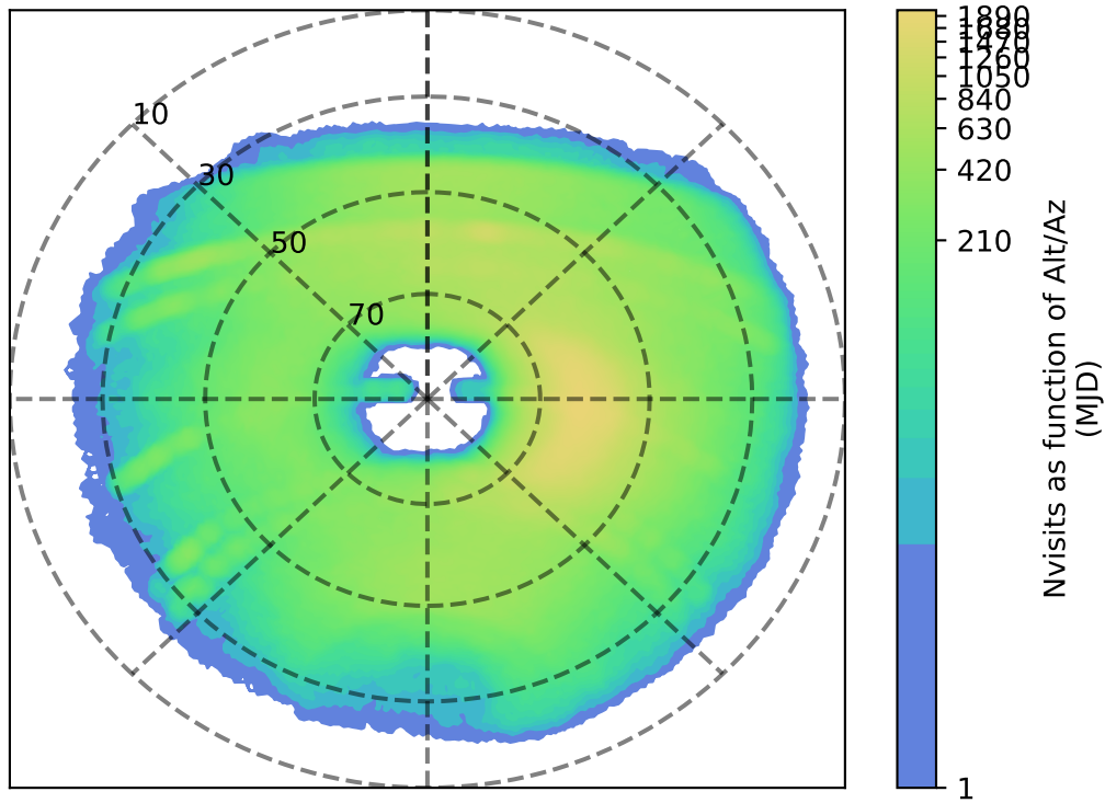
internal_u_expt38_nscale1.1v3.4_10yrs y: Nvisits as function of Alt/Az
