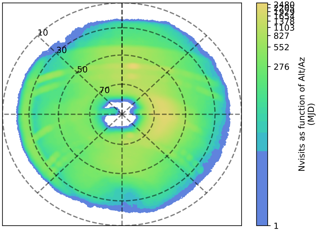
internal_u_expt38_nscale1.1v3.4_10yrs r: Nvisits as function of Alt/Az
