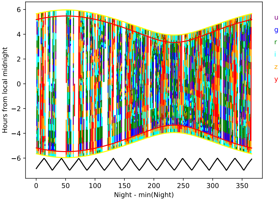
internal_u_expt38_nscale1.1v3.4_10yrs year 8-9: Hourglass
