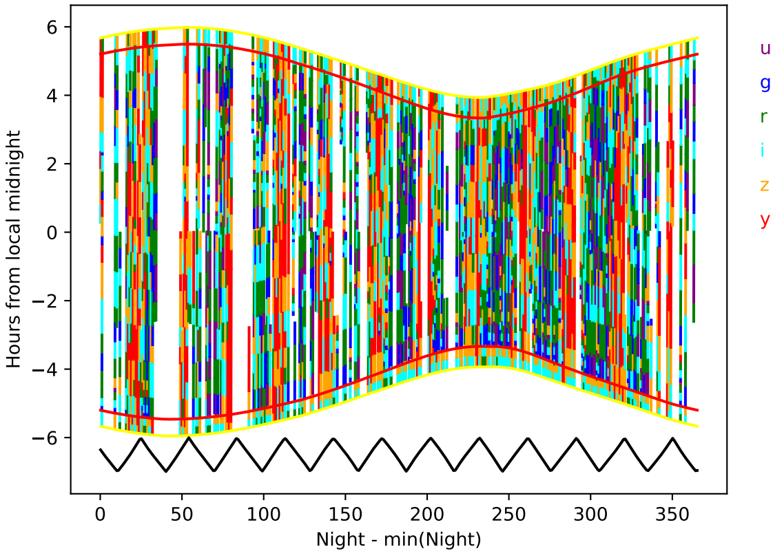
internal_u_expt38_nscale1.1v3.4_10yrs year 4-5: Hourglass
