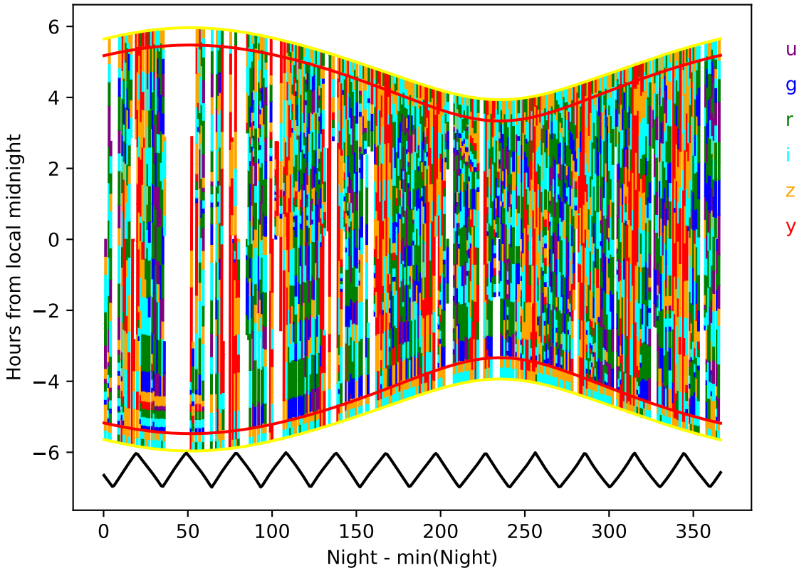
internal_u_expt38_nscale1.1v3.4_10yrs year 2-3: Hourglass
