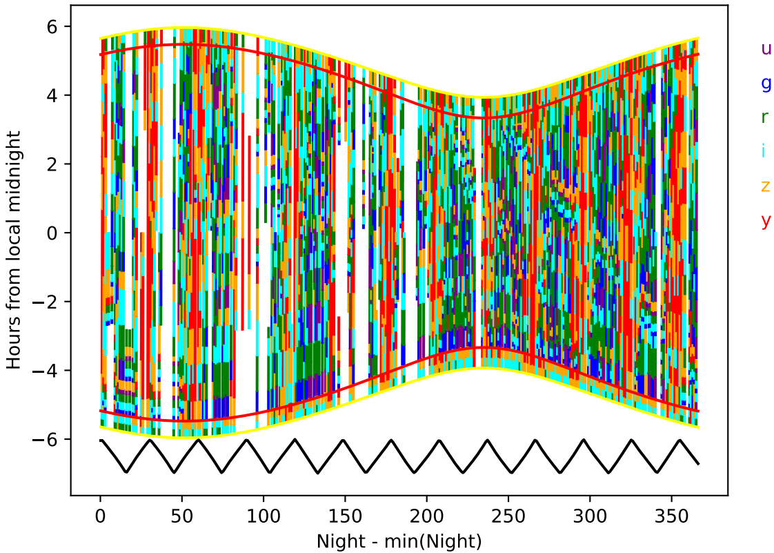
internal_u_expt38_nscale1.1v3.4_10yrs year 1-2: Hourglass
