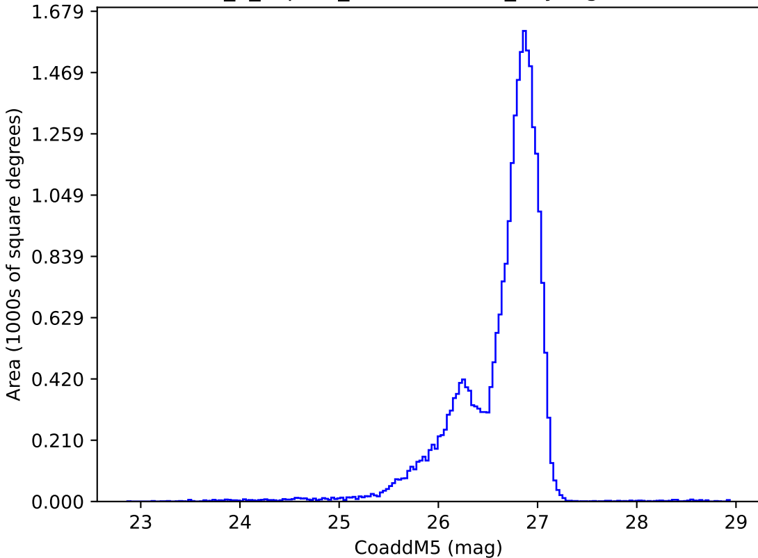
internal_u_expt38_nscale1.1v3.4_10yrs g: CoaddM5
