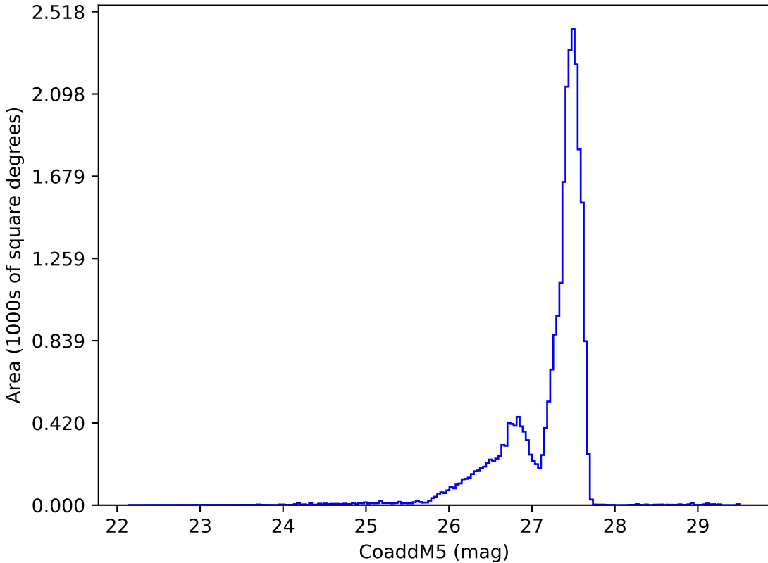
internal_u_expt38_nscale1.1v3.4_10yrs : CoaddM5
