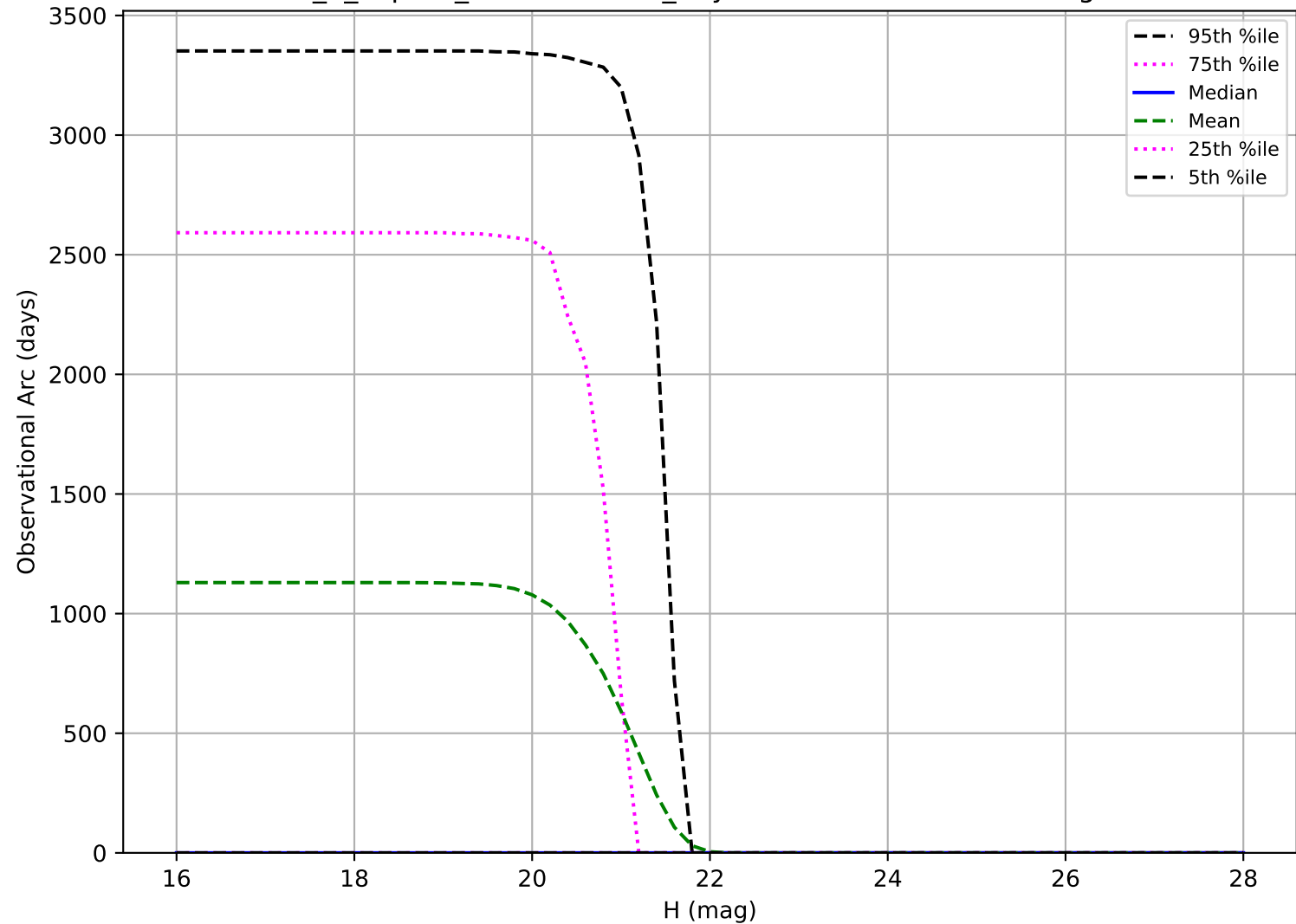
internal_u_expt38_nscale1.0v3.4_10yrs: Observational Arc Length Vatra
