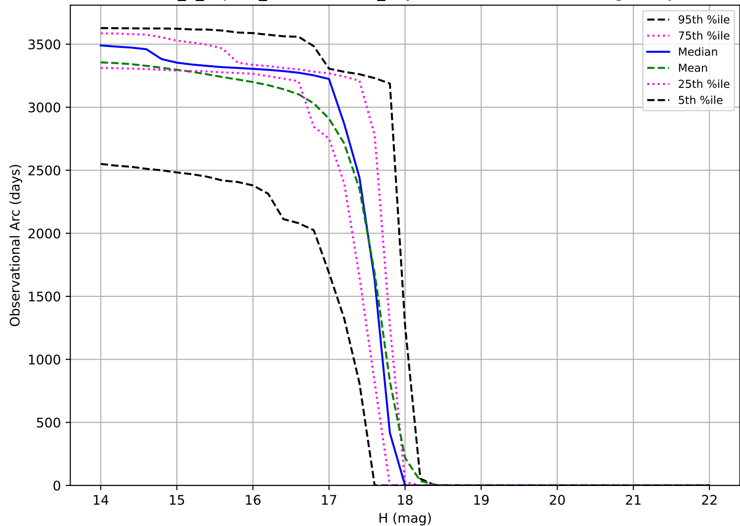
internal_u_expt38_nscale1.0v3.4_10yrs: Observational Arc Length Trojan
