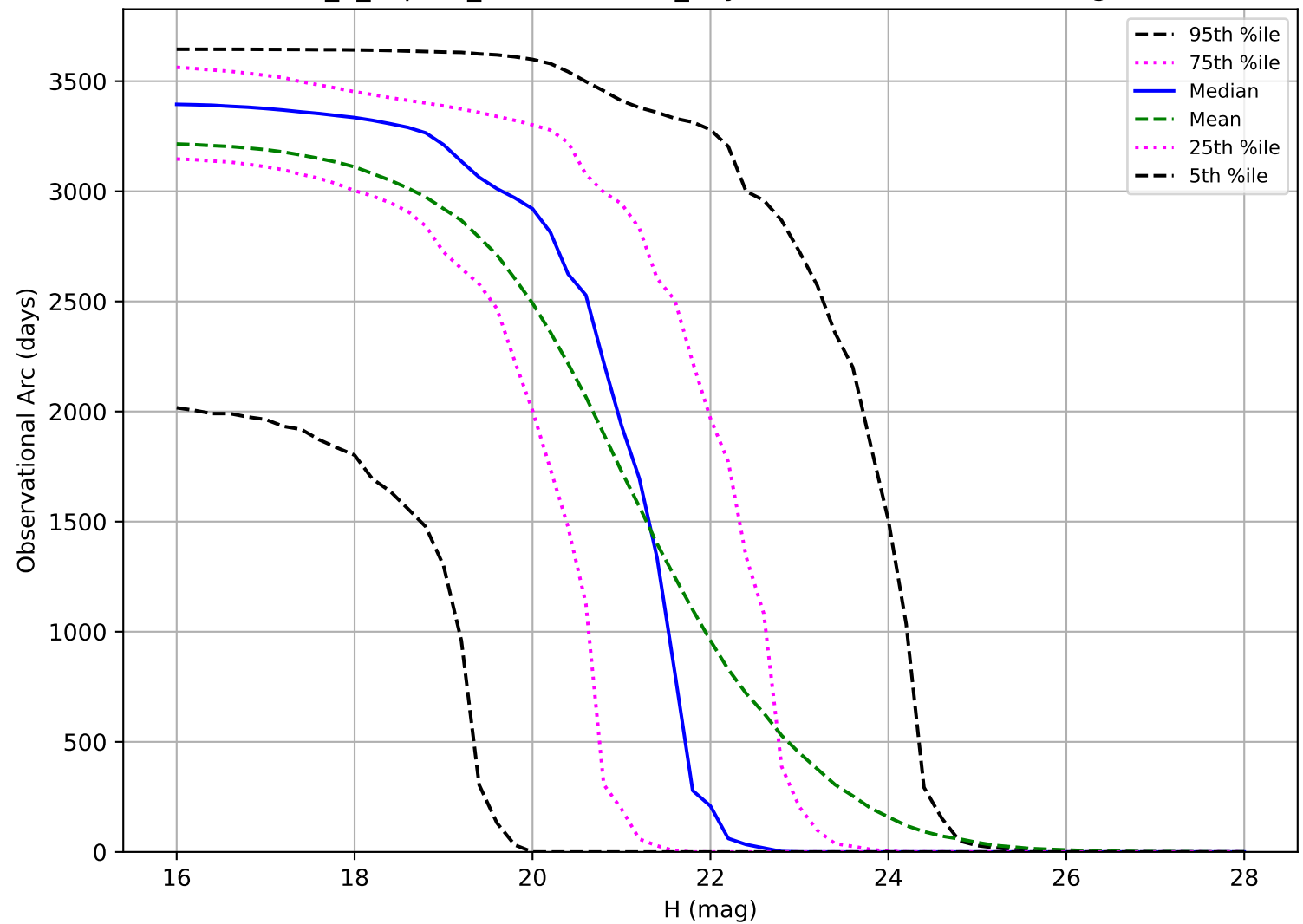
internal_u_expt38_nscale1.0v3.4_10yrs: Observational Arc Length PHA
