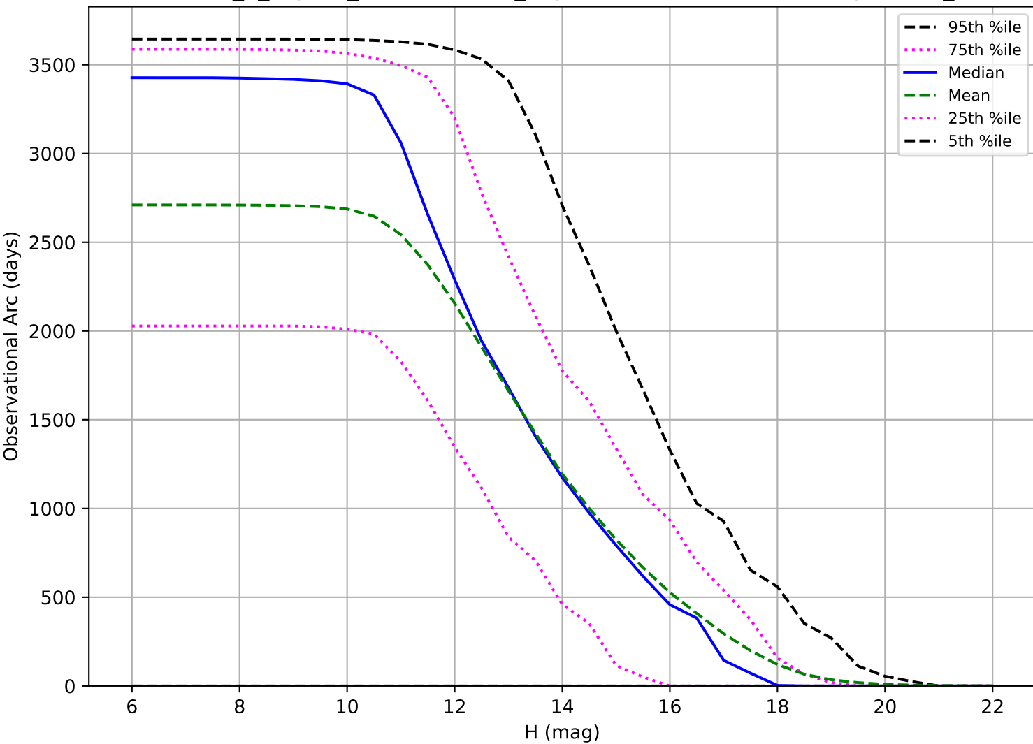
internal_u_expt38_nscale1.0v3.4_10yrs: Observational Arc Length OCC_r5
