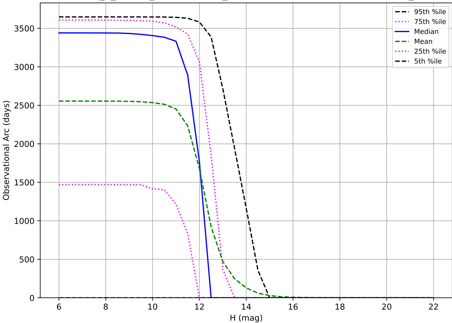
internal_u_expt38_nscale1.0v3.4_10yrs: Observational Arc Length OCC_r20
