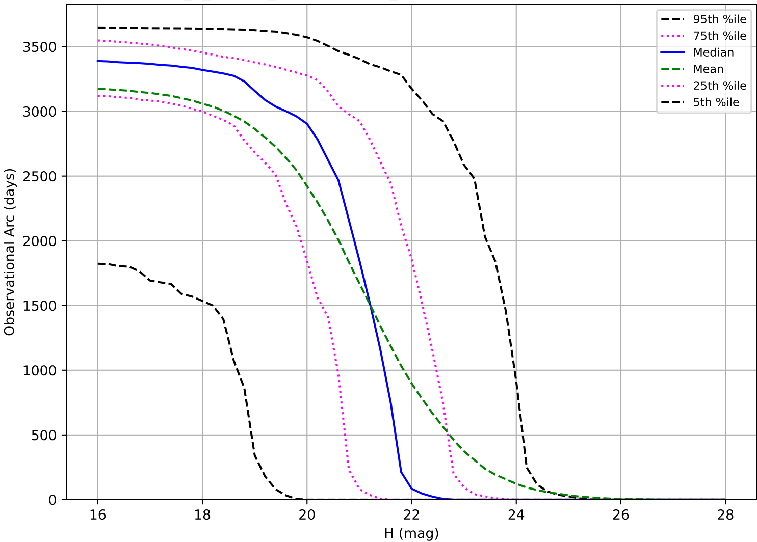
internal_u_expt38_nscale1.0v3.4_10yrs: Observational Arc Length NEO
