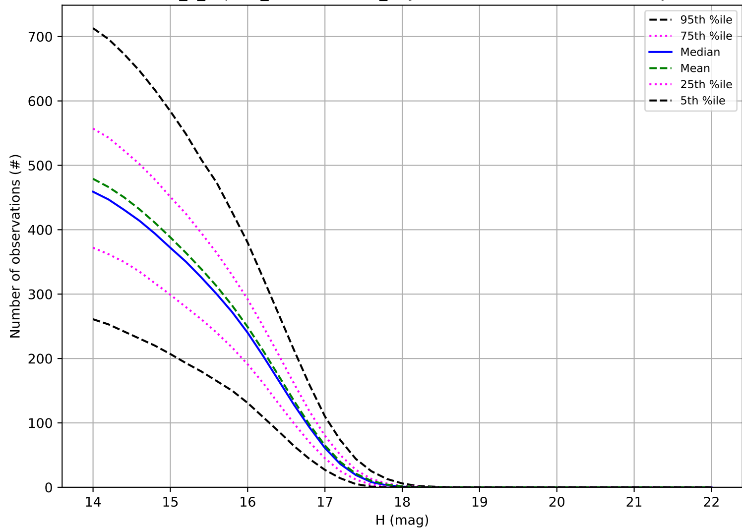
internal_u_expt38_nscale1.0v3.4_10yrs: Number of observations Trojan
