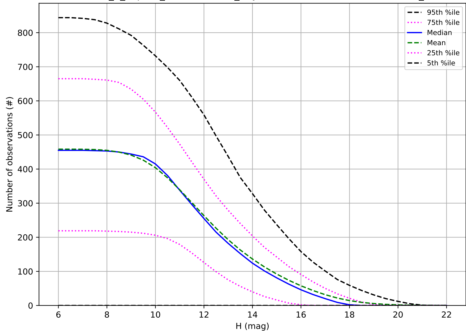
internal_u_expt38_nscale1.0v3.4_10yrs: Number of observations OCC_r5
