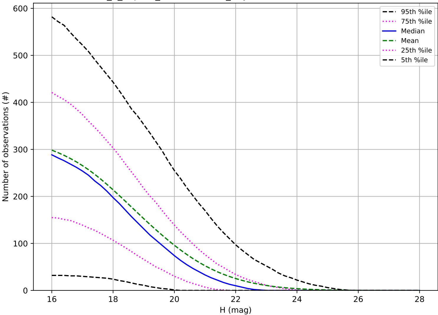
internal_u_expt38_nscale1.0v3.4_10yrs: Number of observations NEO
