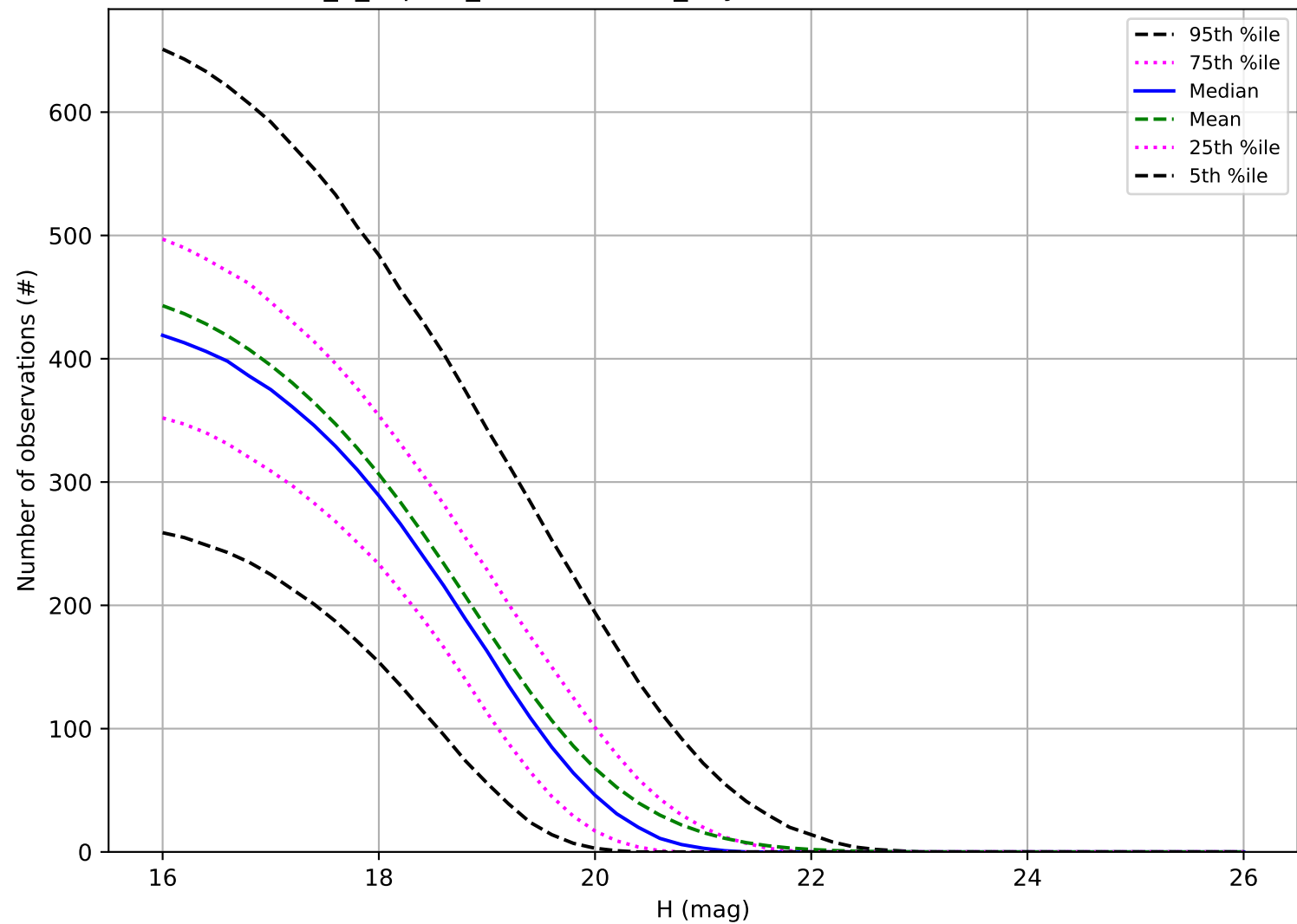
internal_u_expt38_nscale1.0v3.4_10yrs: Number of observations MBA
