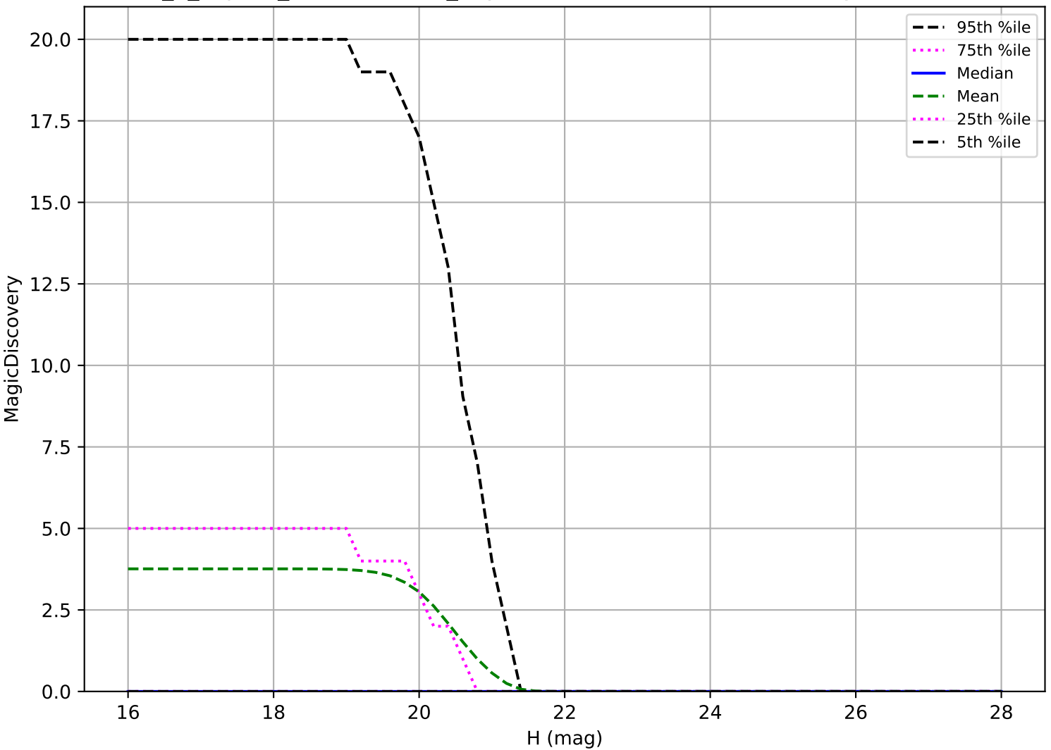
internal_u_expt38_nscale1.0v3.4_10yrs: Vatira 6 detections in 60 nights detection loss
