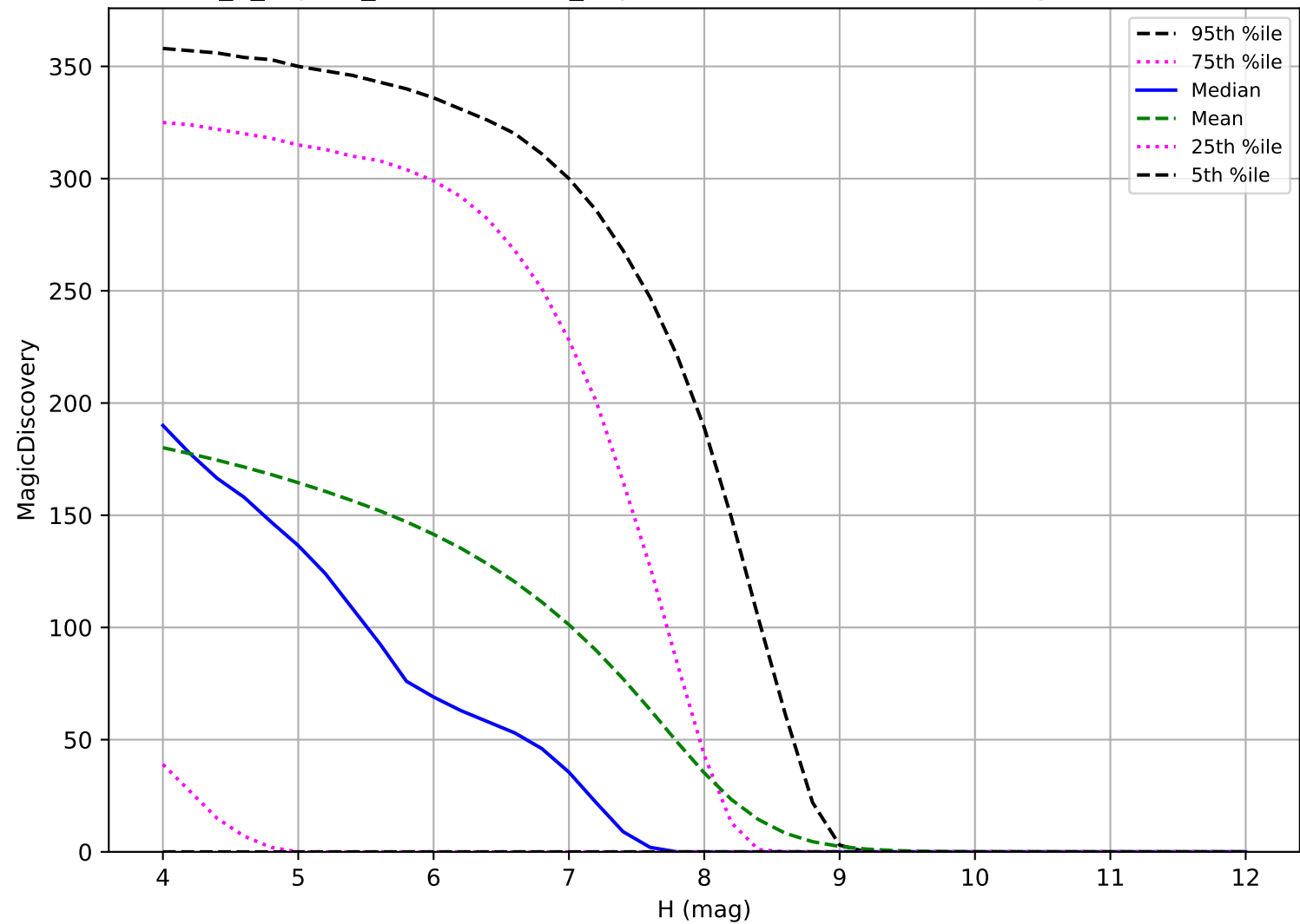
internal_u_expt38_nscale1.0v3.4_10yrs: TNO 6 detections in 60 nights detection loss
