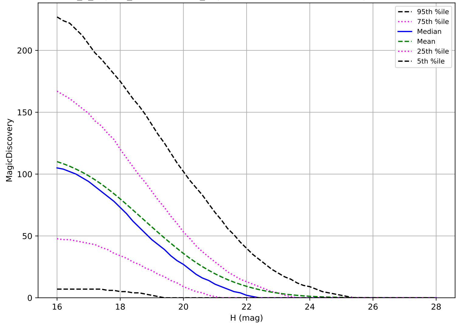
internal_u_expt38_nscale1.0v3.4_10yrs: PHA 6 detections in 60 nights detection loss
