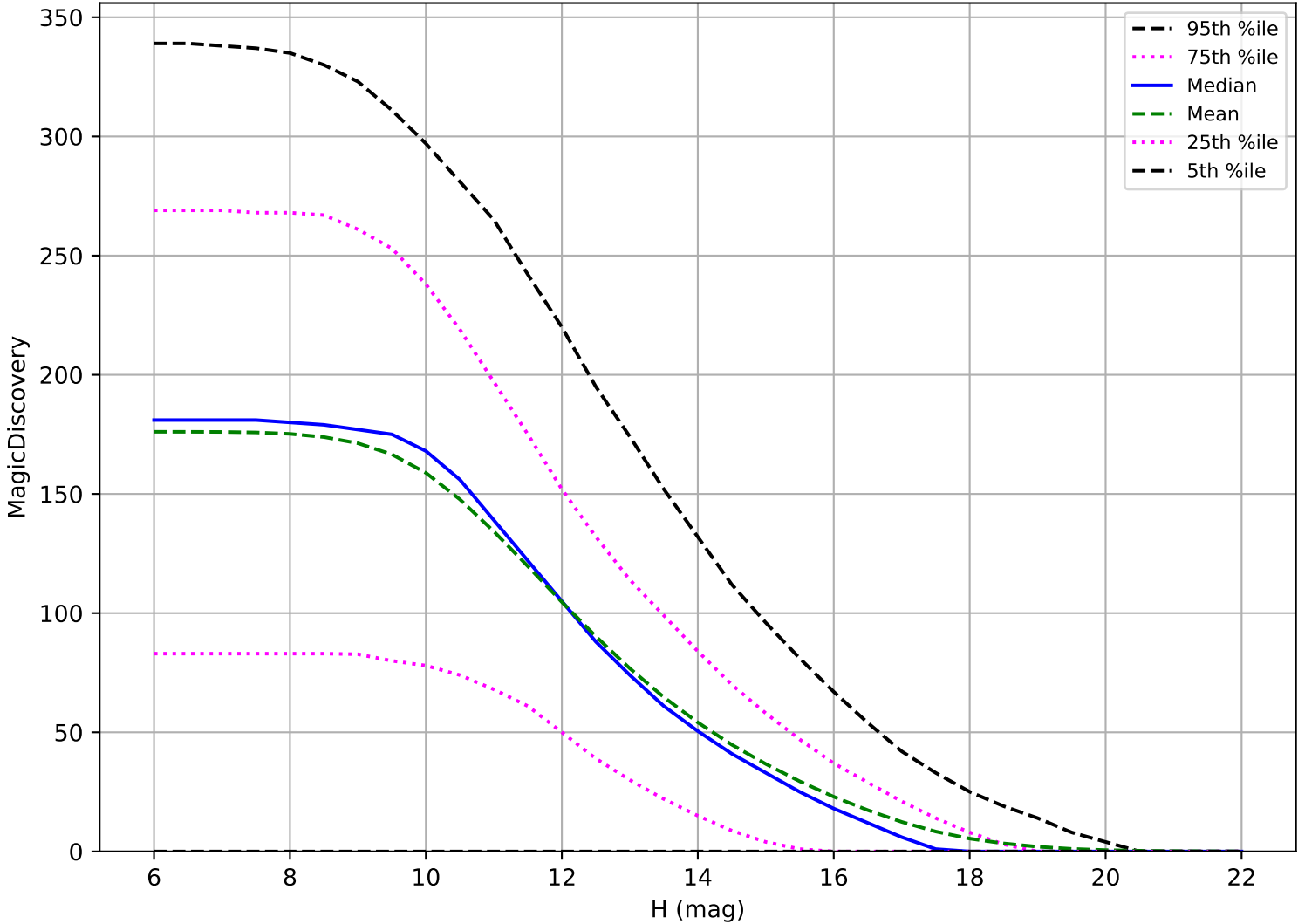
internal_u_expt38_nscale1.0v3.4_10yrs: OCC_r5 6 detections in 60 nights detection loss
