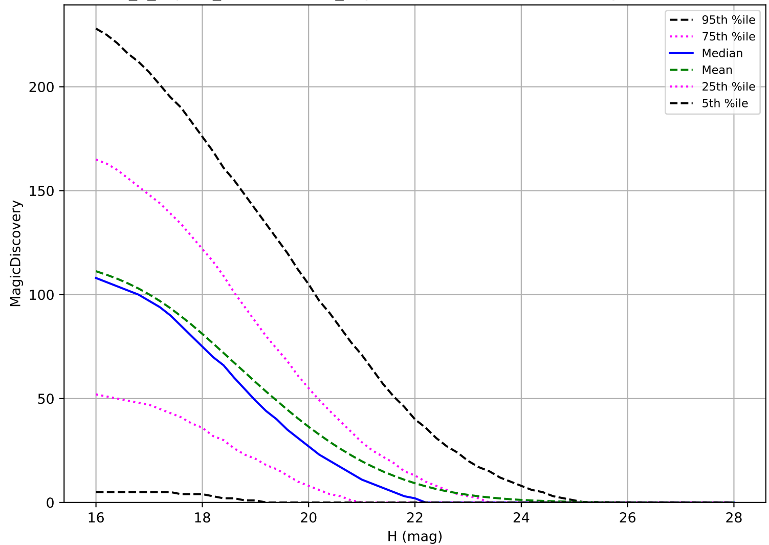
internal_u_expt38_nscale1.0v3.4_10yrs: NEO 6 detections in 60 nights detection loss
