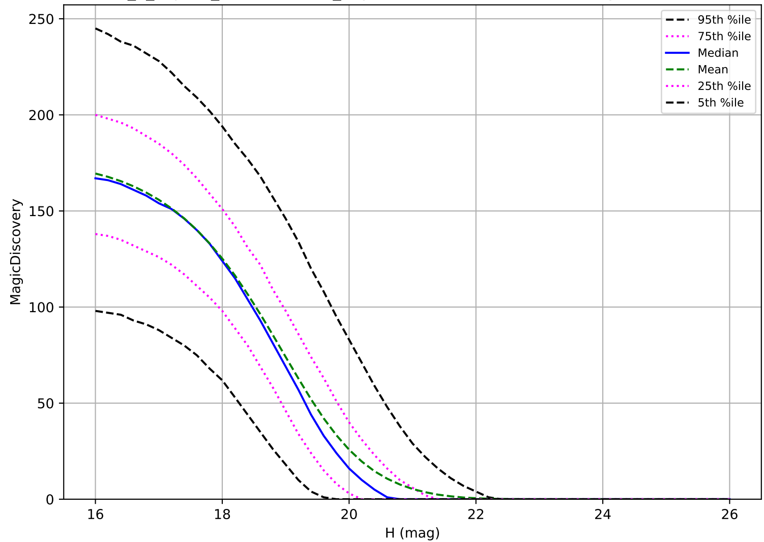
internal_u_expt38_nscale1.0v3.4_10yrs: MBA 6 detections in 60 nights detection loss
