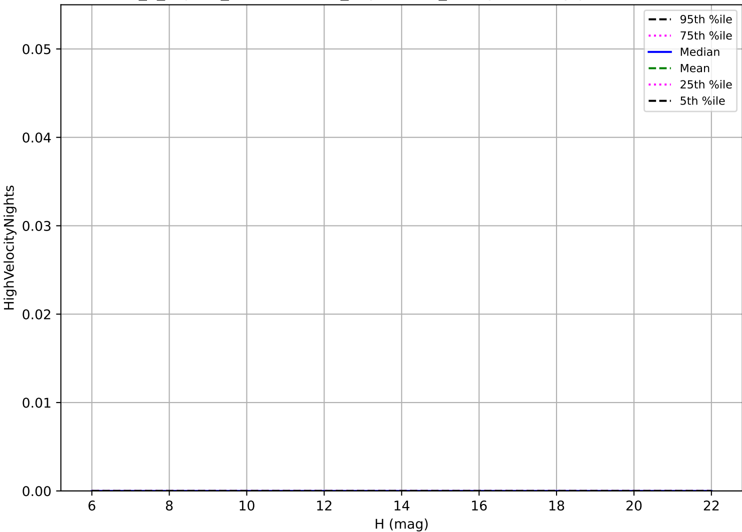
internal_u_expt38_nscale1.0v3.4_10yrs: OCC_r5 High velocity pair detection loss
