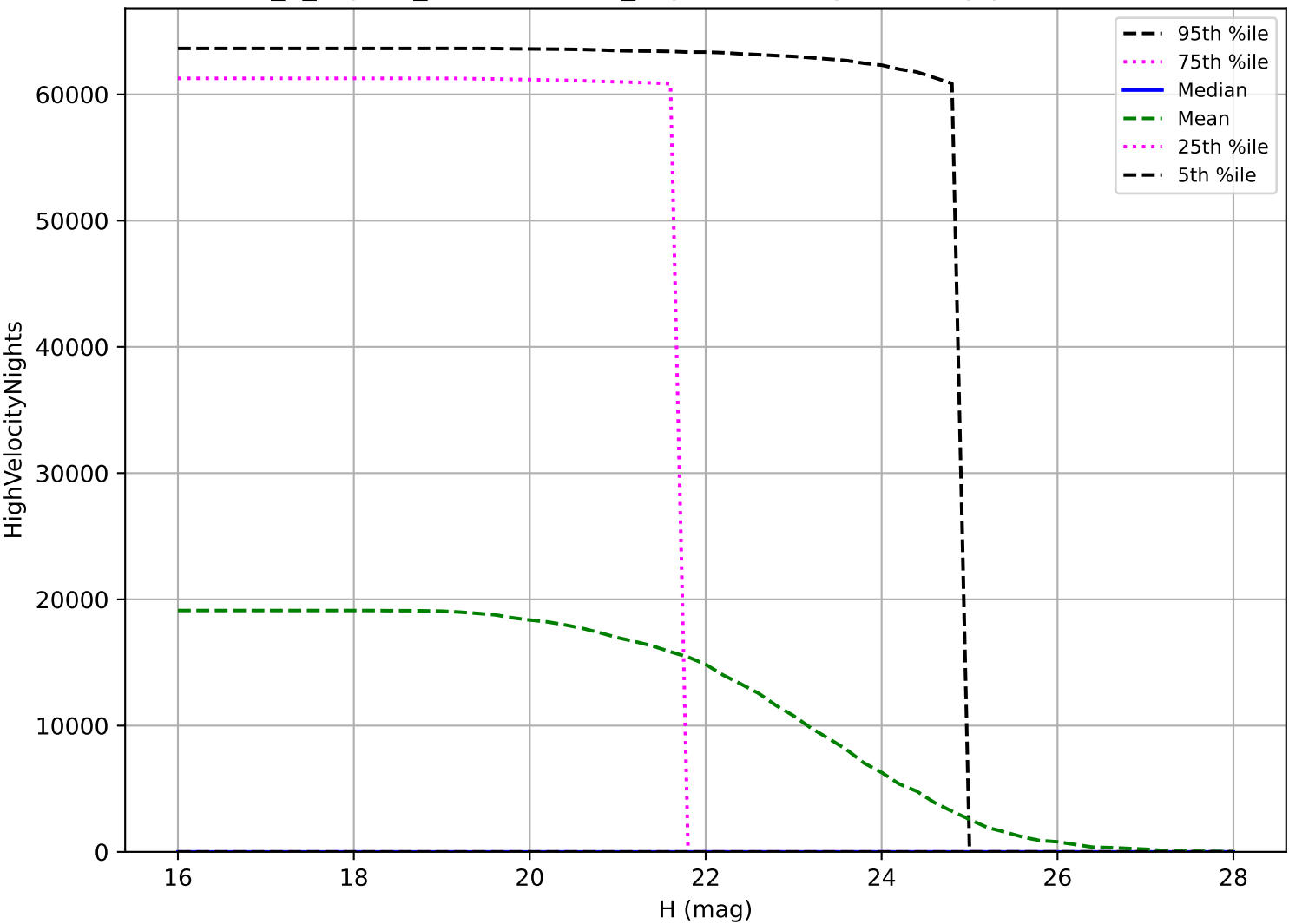
internal_u_expt38_nscale1.0v3.4_10yrs: NEO High velocity pair detection loss
