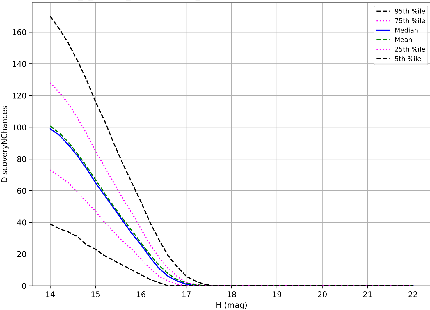
internal_u_expt38_nscale1.0v3.4_10yrs: Trojan 3 pairs in 15 nights detection loss
