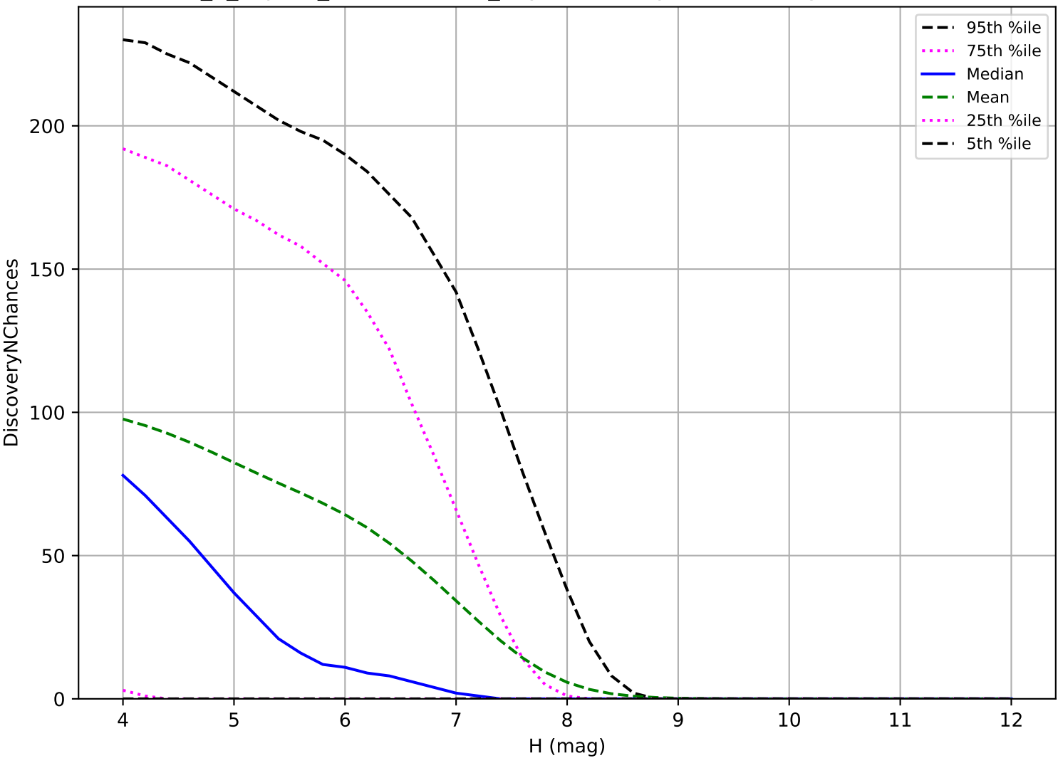
internal_u_expt38_nscale1.0v3.4_10yrs: TNO 3 pairs in 15 nights detection loss
