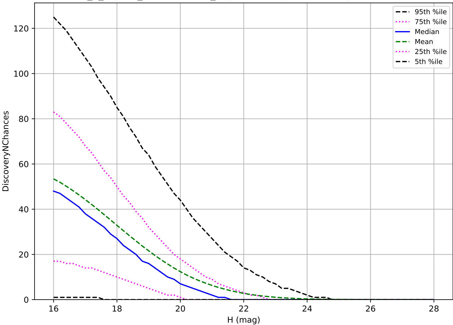
internal_u_expt38_nscale1.0v3.4_10yrs: PHA 3 pairs in 15 nights detection loss
