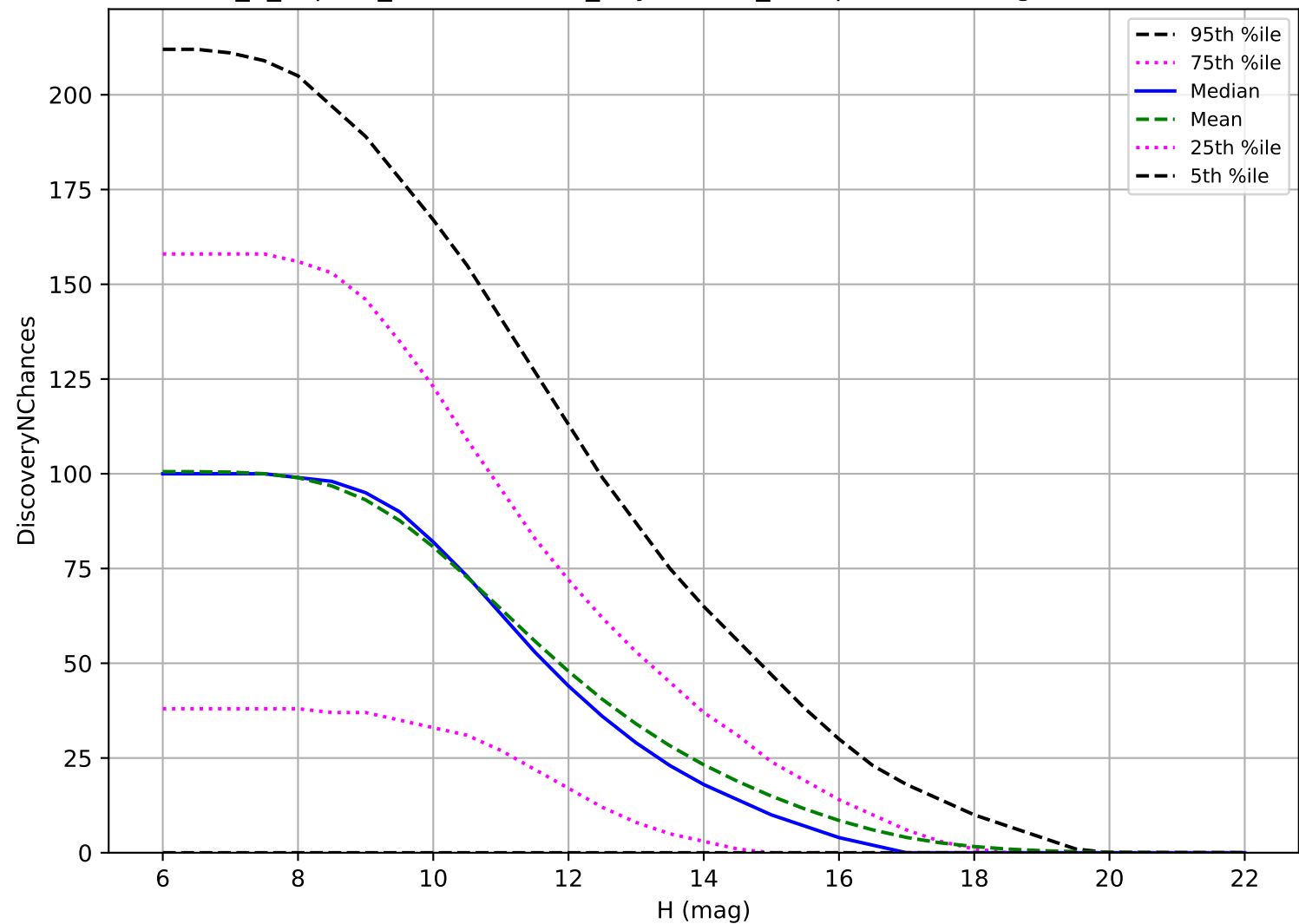
internal_u_expt38_nscale1.0v3.4_10yrs: OCC_r5 3 pairs in 15 nights detection loss
