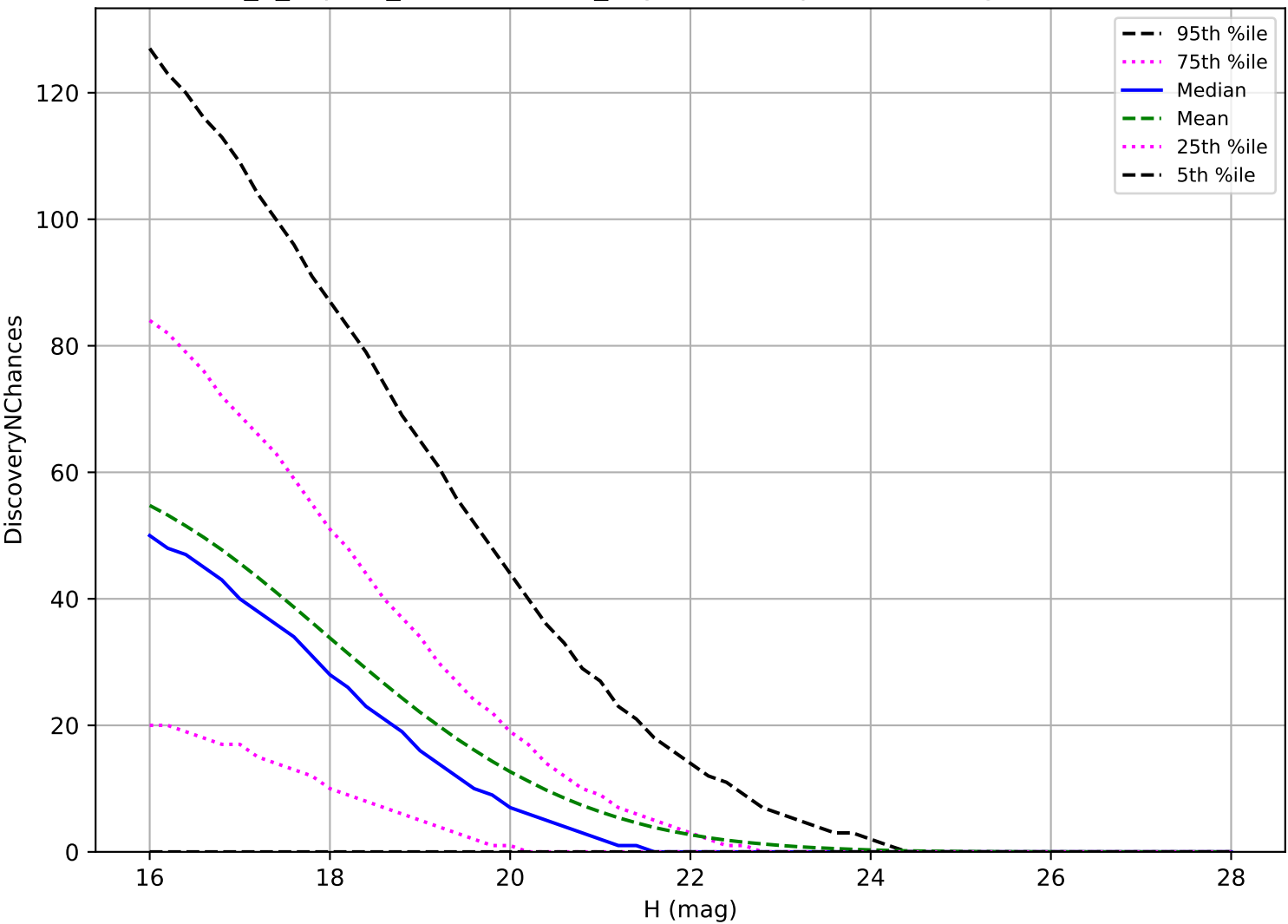
internal_u_expt38_nscale1.0v3.4_10yrs: NEO 3 pairs in 15 nights detection loss
