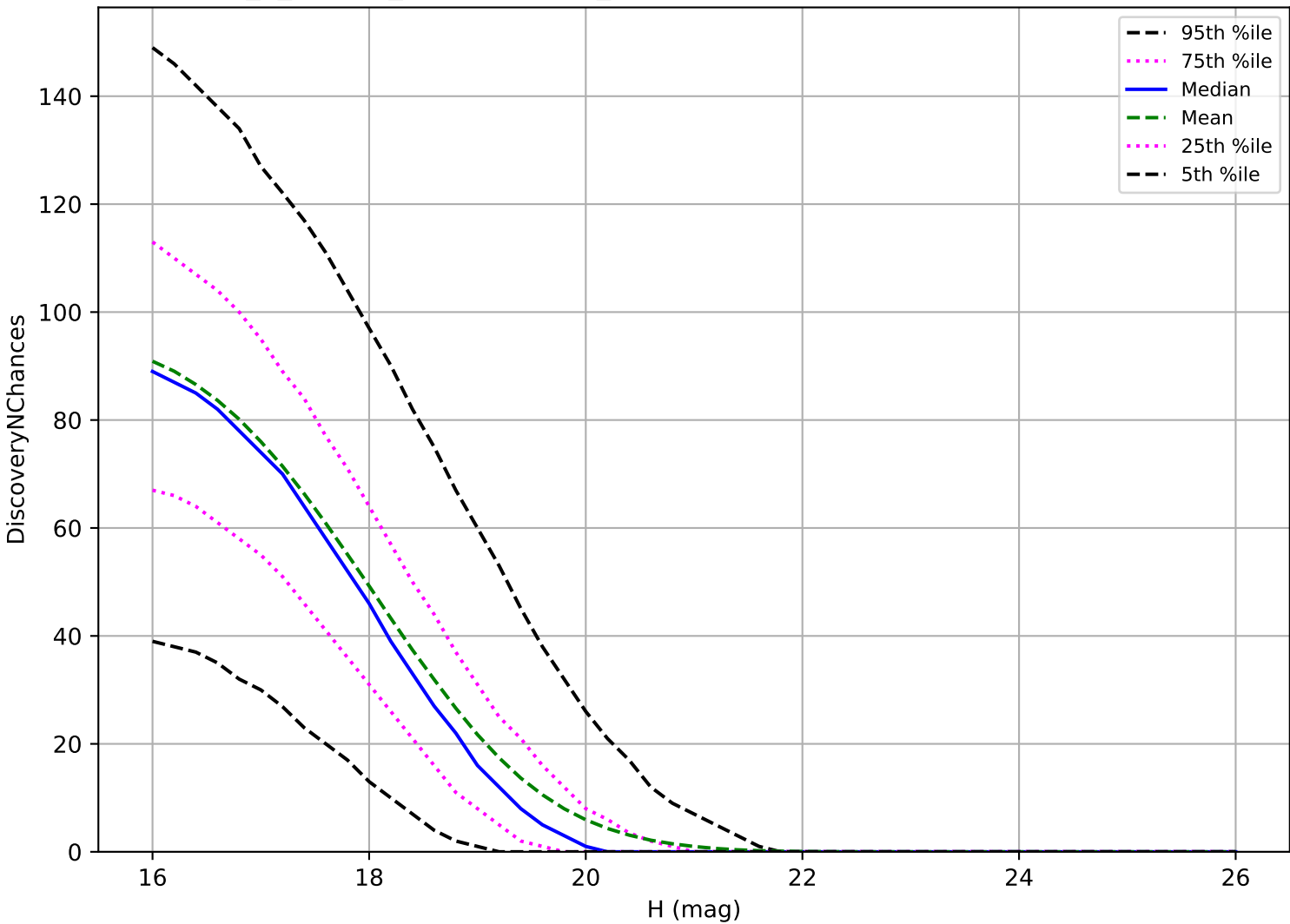
internal_u_expt38_nscale1.0v3.4_10yrs: MBA 3 pairs in 15 nights detection loss
