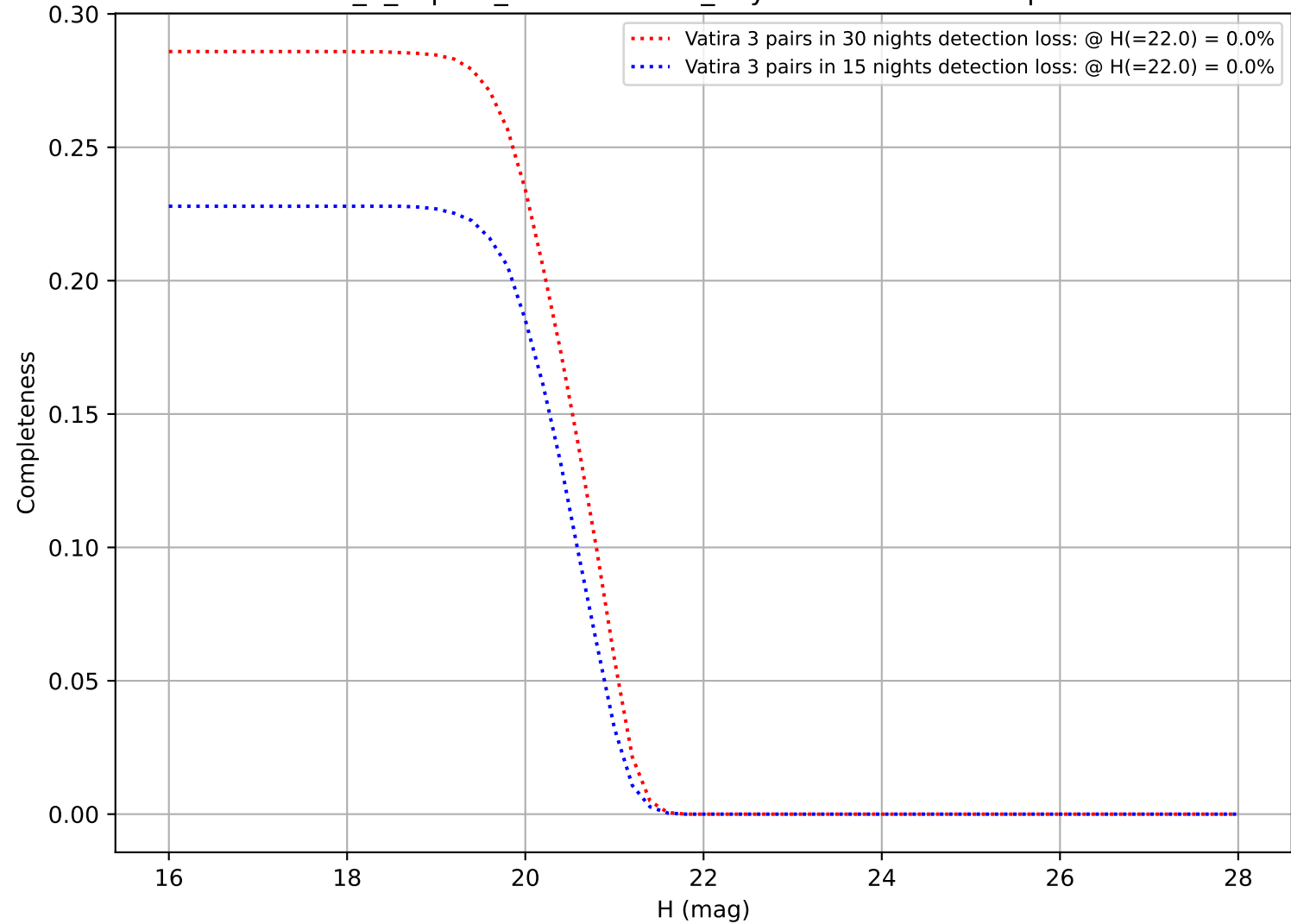
internal_u_expt38_nscale1.0v3.4_10yrs: DifferentialCompleteness
