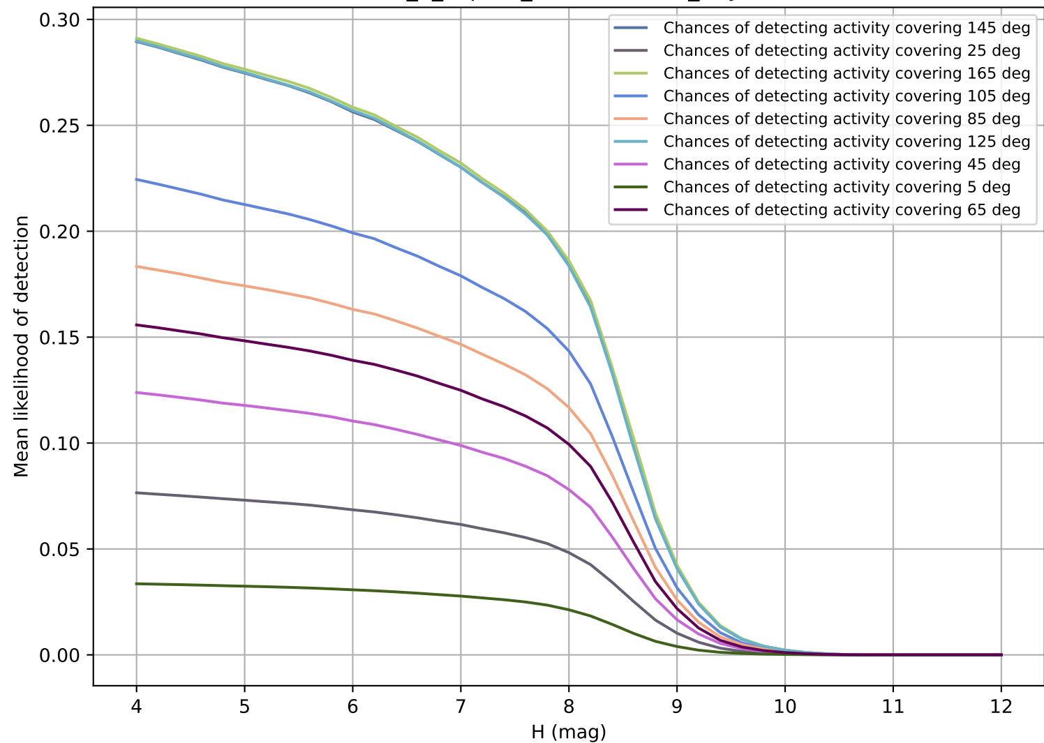
internal_u_expt38_nscale1.0v3.4_10yrs TNO
