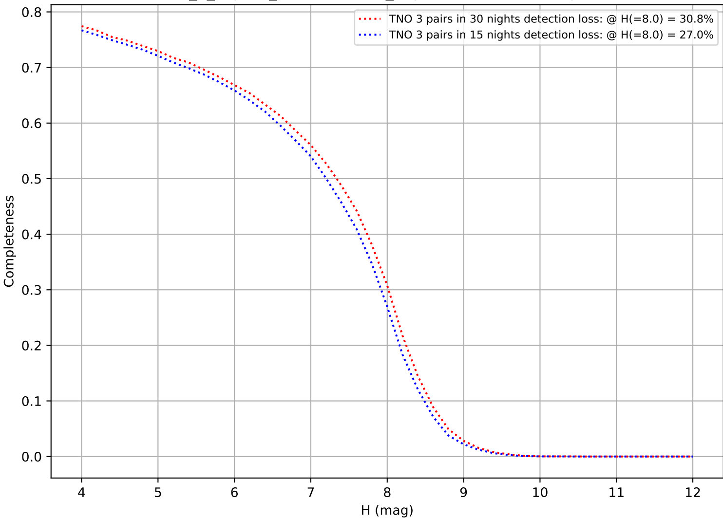
internal_u_expt38_nscale1.0v3.4_10yrs: DifferentialCompleteness
