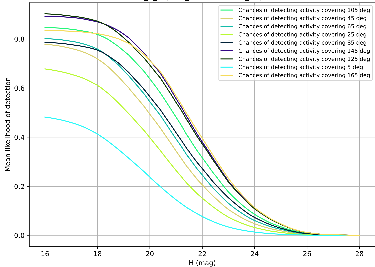
internal_u_expt38_nscale1.0v3.4_10yrs NEO
